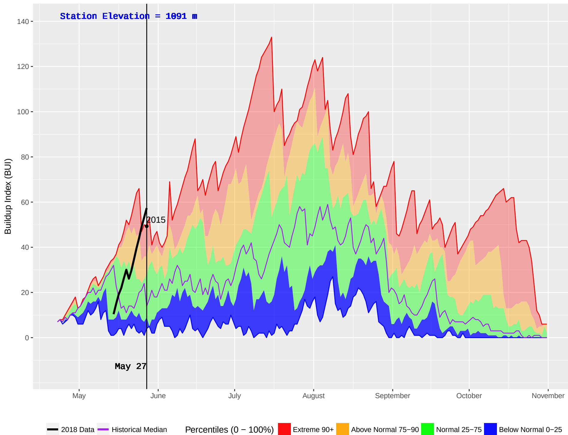
BIG MOUTH 2 (868) : Historical (2004–2016) and Current (2018) Noon Buildup Index (BUI)
