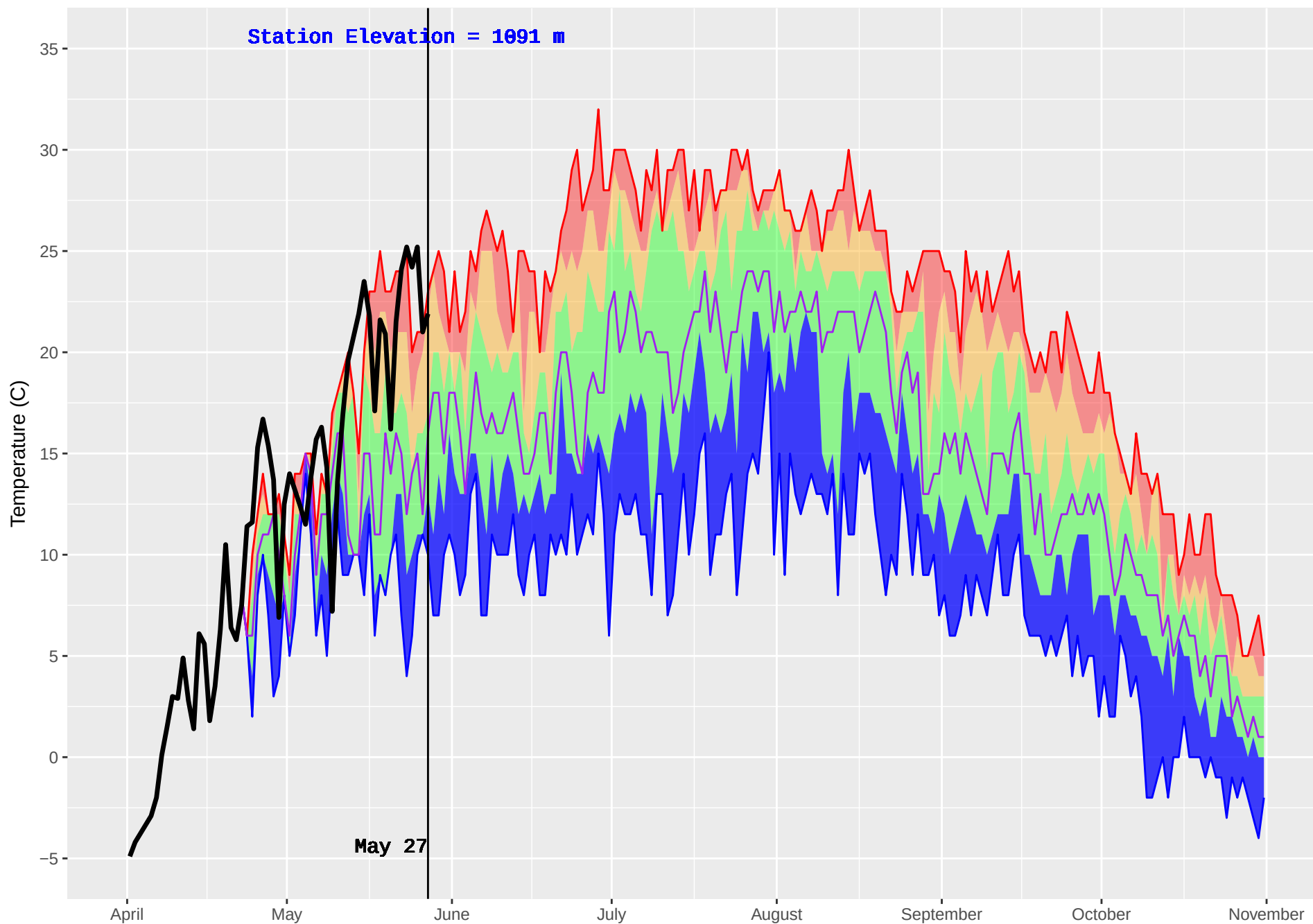
BIG MOUTH 2 (868) : Historical (2004–2016) and Current (2018) Noon Temperature
