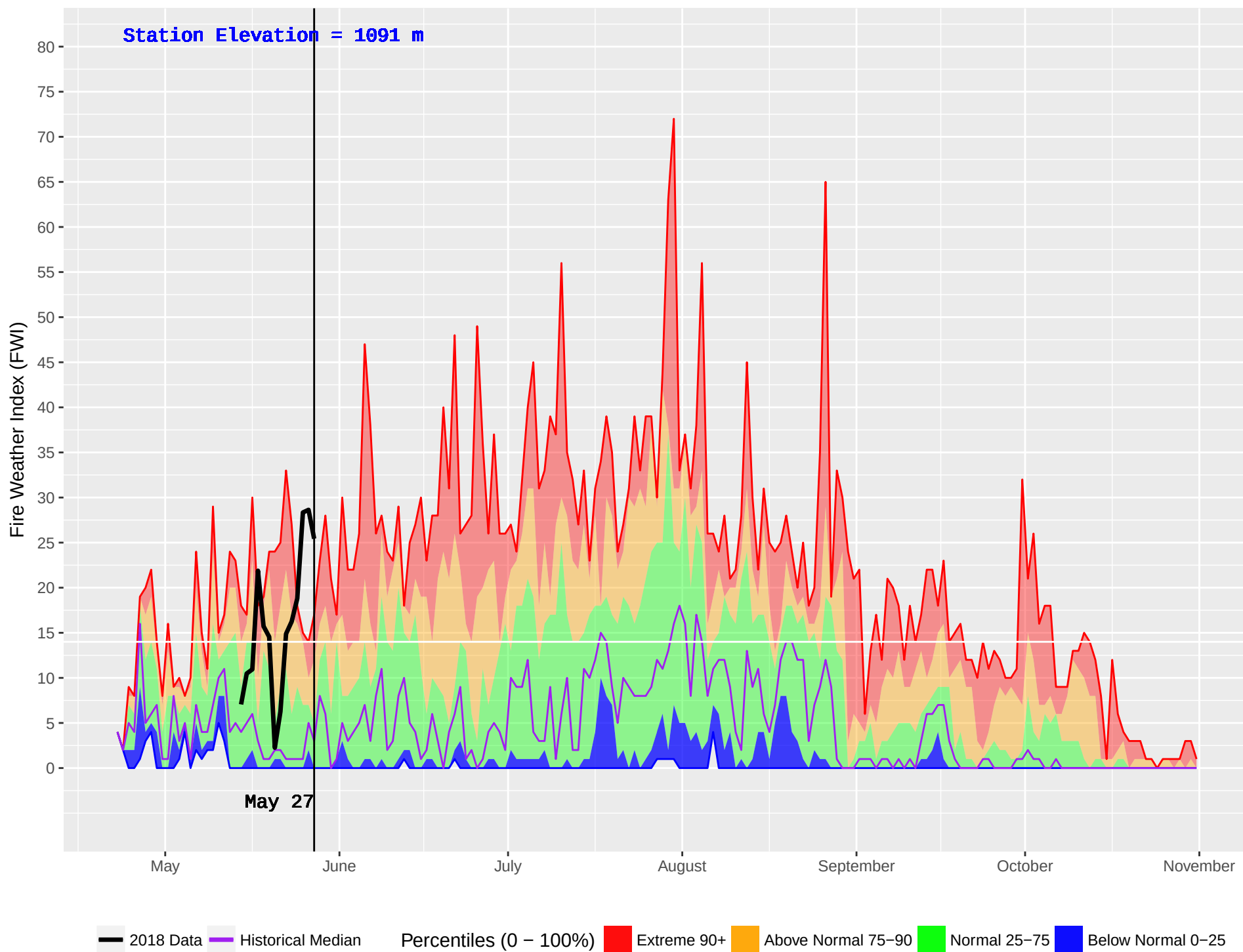
BIG MOUTH 2 (868) : Historical (2004–2016) and Current (2018) Noon Fire Weather Index (FWI)
