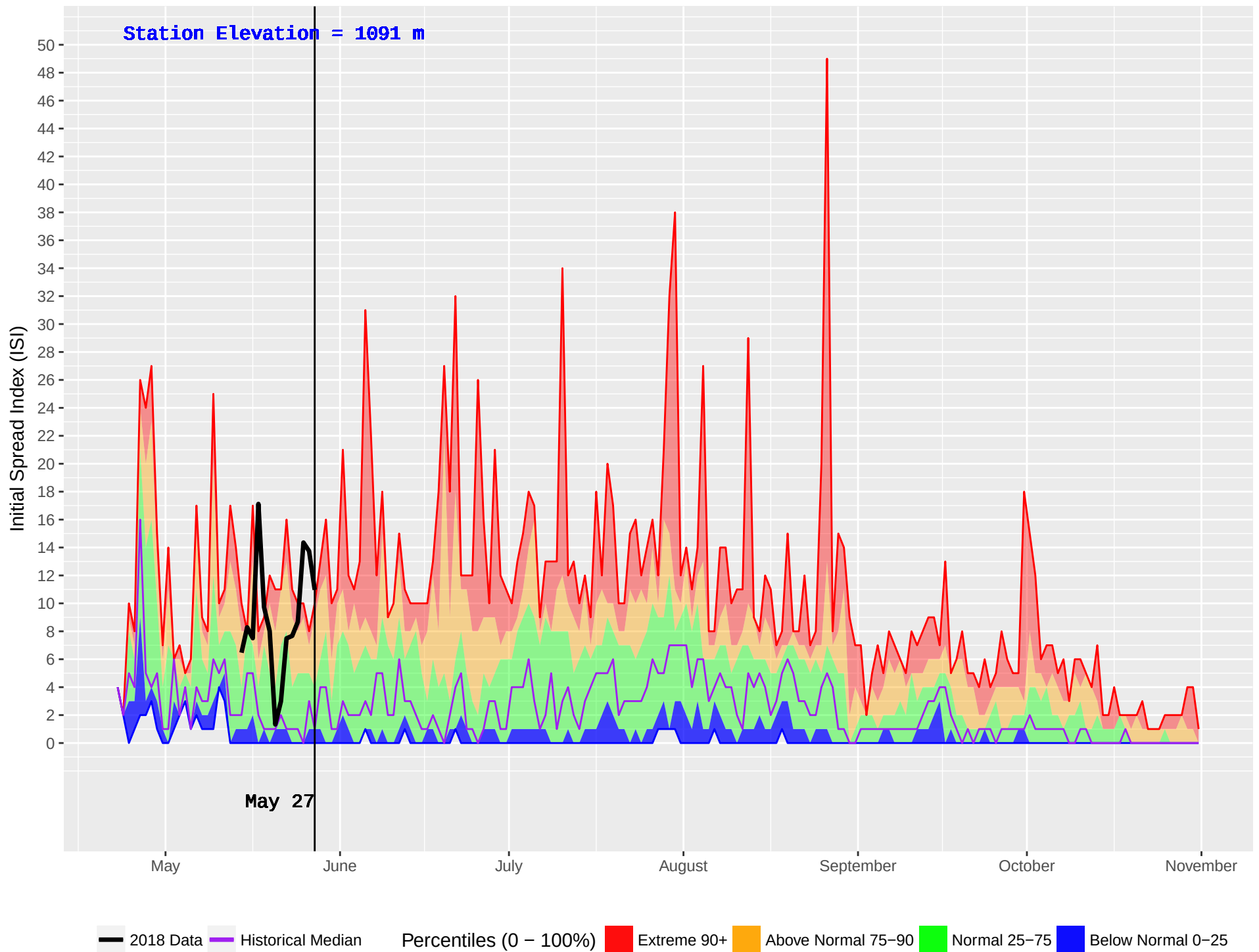
BIG MOUTH 2 (868) : Historical (2004–2016) and Current (2018) Noon Initial Spread Index (ISI)
